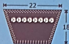
SECTION SPC
