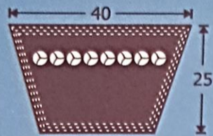
SECTION E/40
