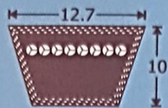
SECTION SPA
