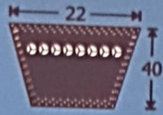
SECTION C/22
