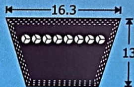
SECTION SPB
